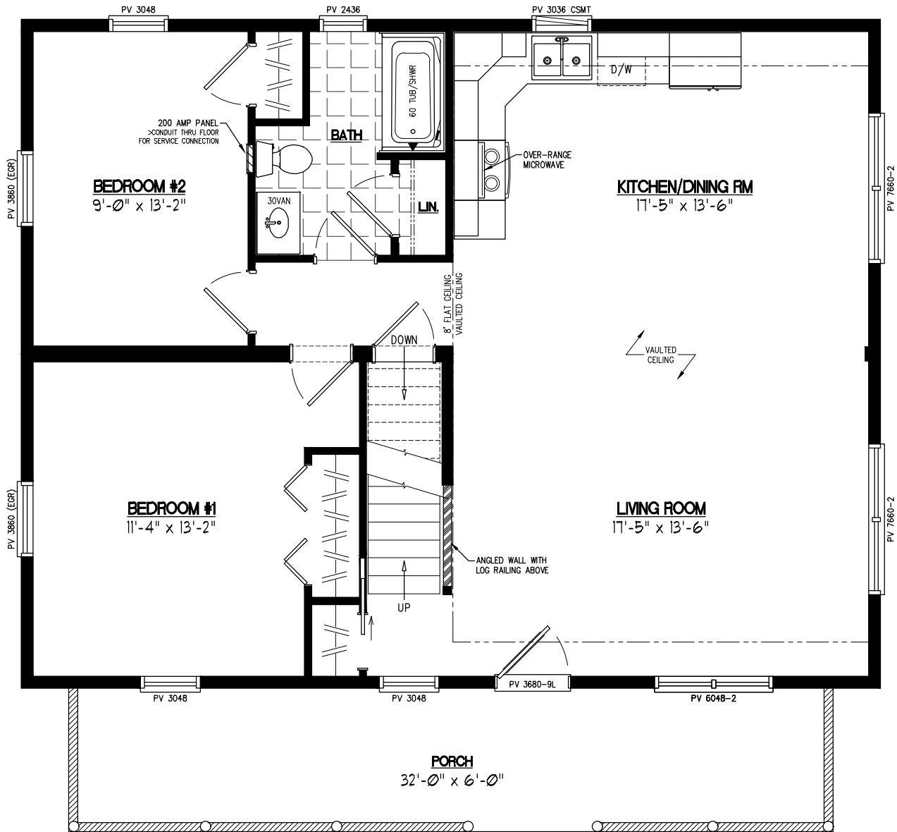
28x36 MOUNTAINEER DELUXE Plan #28MD1402
