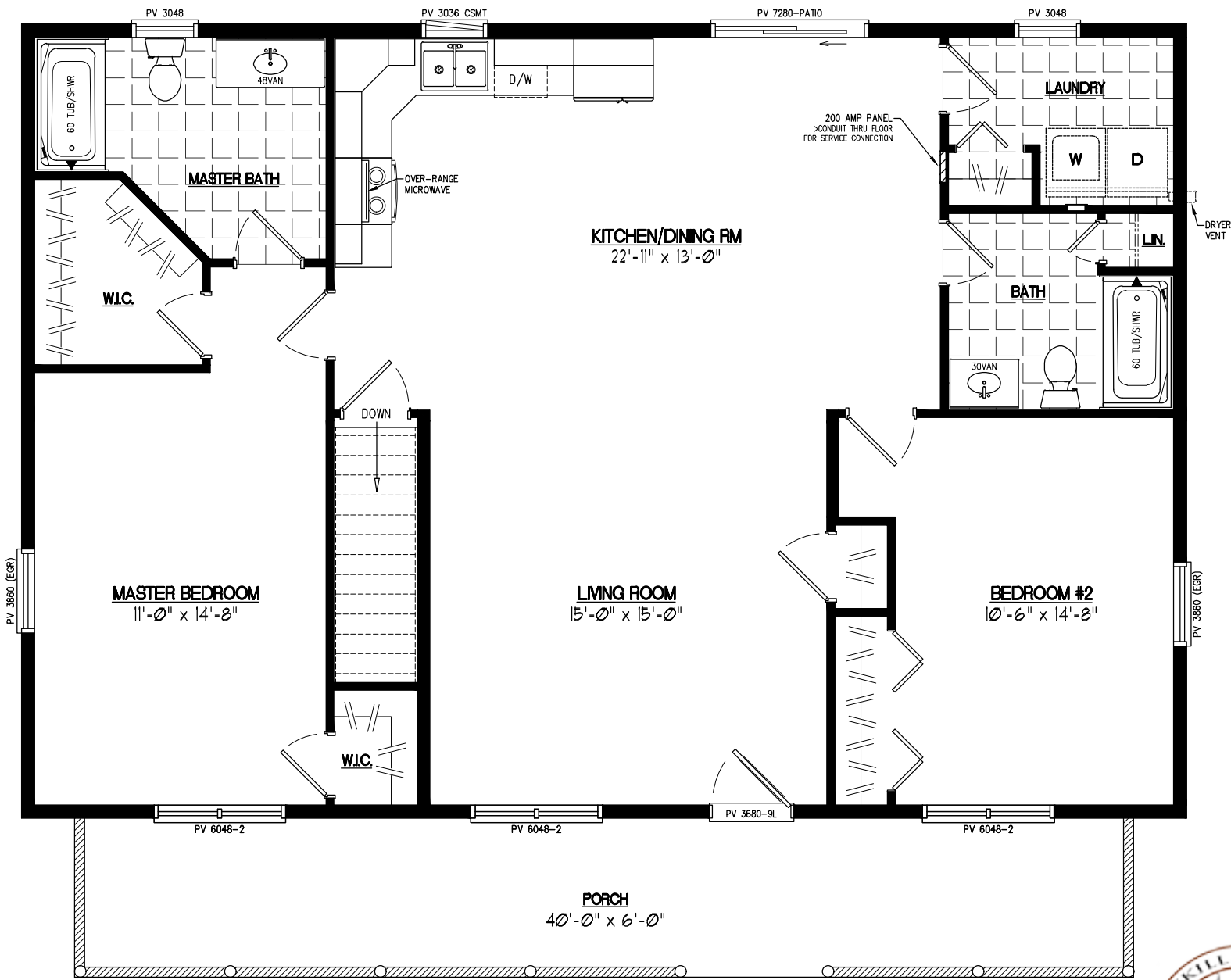
30x44 MUSKETEER Plan #30MK1504
